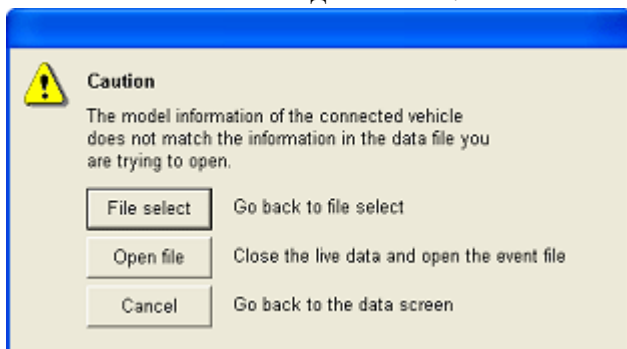
Caution Dialog
