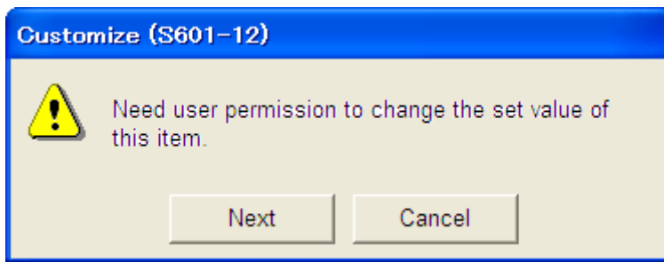
Caution Dialog
