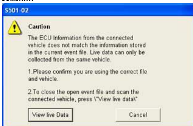
Caution Dialog
