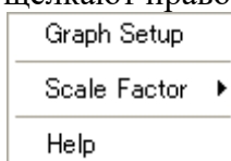
Popup Menu
