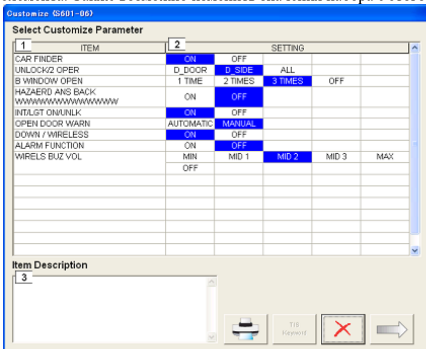
Customize Dialog
